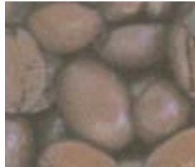
Java Beans
